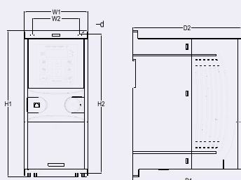
Wall mounting of 0.75~2.2kW VFDs
